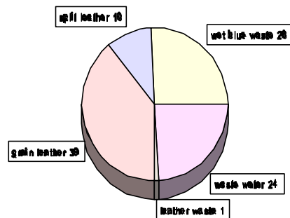
Figure 19. Chrome distribution in leather, solid waste and effluent (expressed as % of \text{Cr}_2\text{O}_3 offer)
